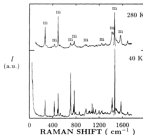
FIG. 1. Unpolarized Raman spectra of single-crystal C_{60} in the fcc phase ( T=280\text{ K} , upper curve) and in the sc phase ( T=40\text{ K} , lower curve). The peaks at \sim 1467\text{ cm}^{-1} are scaled down by a factor of 6. The predicted modes for the free molecule are indicated with an "m."
