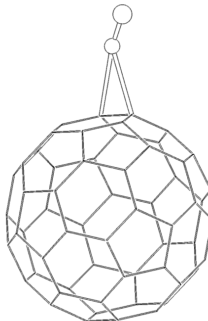
FIG. 3. Relative orientations of C_{60} and CO molecules in the (CO)_x C_{60} crystal, as resulted from the best fit.
