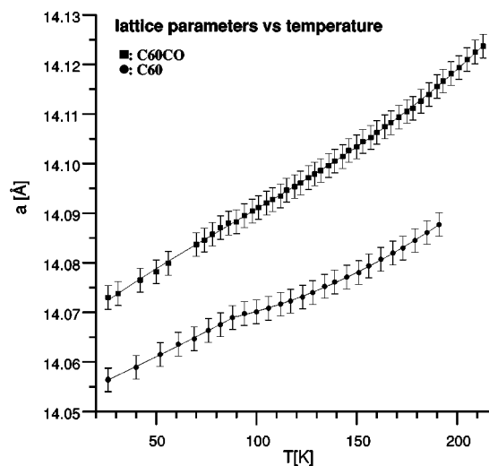
FIG. 1. The cubic lattice constant of (CO) x C 60 and C 60 as a function of the temperature. The values were determined from the varying position of a single peak, and they were not corrected for the zero-point error. Error bars pertain to the standard deviations including the zero-point error. Relative values within one temperature run will be much more accurate, as the same zero-point error applies for all data points from a single run. The lines are a guide for the eye.
