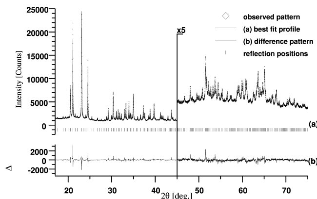
FIG. 2. Experimental data and the fit through the x-ray powder diffraction diagram of (\text{CO})_x\text{C}_{60} at T=25 K.
