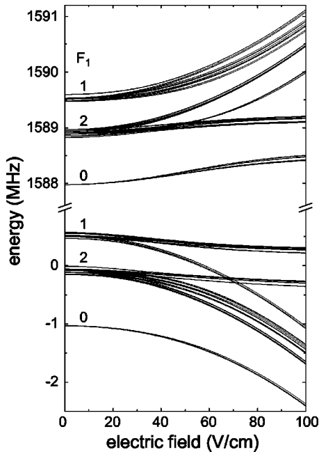
FIG. 6. Calculated Stark shift for the manifold of hyperfine levels of ^{14}\text{ND}_3 in electric fields up to 100 V/cm.
