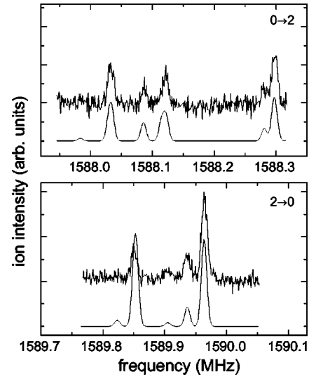
FIG. 4. The weak F'_1 = 0 \rightarrow F''_1 = 2 and F'_1 = 2 \rightarrow F''_1 = 0 transitions for ^{14}\text{ND}_3 , recorded at increased rf powers of 0.25 mW and 0.13 mW, respectively. Underneath the experimental spectra, the simulated spectra are shown.
