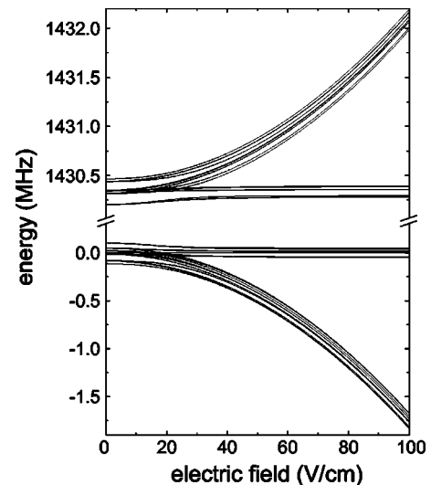
FIG. 8. Calculated Stark shift for the manifold of hyperfine levels of ^{15}\text{ND}_3 in electric fields up to 100 V/cm.
