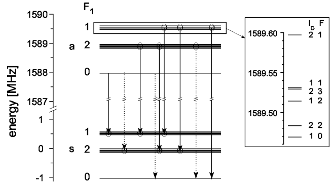
FIG. 5. Energy-level structure of 14 ND 3 ( |J,K\rangle=|1,1\rangle ). The quadrupole interaction of the 14 N atom causes the main splitting of both the upper and the lower component of the inversion doublet in three levels, labeled with the quantum number F_1 . The nuclear spins of the deuterium atoms cause additional splittings, shown enlarged for the F_1=1 component at the right-hand side of the figure. The strong (weak) F_1' \rightarrow F_1'' transitions observed in the experimental spectra are indicated by solid (dashed) arrows.
