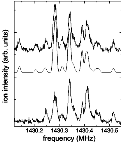
FIG. 7. High-resolution pure inversion spectra of ^{15}\text{ND}_3 ( |J,K\rangle=|1,1\rangle ), measured by probing the lower inversion level. The upper experimental spectrum is recorded while operating the hexapole in the pulsed mode, and is shown together with the theoretical spectrum obtained from the best fit to the experimental data. The lower experimental spectrum is recorded when the molecules leave the hexapole adiabatically.
