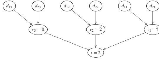
Fig. 5 Inference with noisy-MAX. Observed test value t = 2 implies that the outcome of v_3 = 0 , and v_2 = 2 . The observed test value does not give any information about v_1 .
