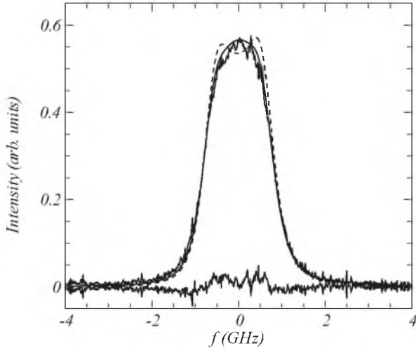
FIG. 10. Coherent Rayleigh-Brillouin scattering on an equimolar mixture of He and Xe (1 bar He and 1 bar Xe) at p = 2 bar (dimensionless pressure \gamma = 1.18 ). Full line shows a prediction of the mixture model by Marquez [8]; dashed line shows a mixture model computed for a single gas of Xe atoms at p = 1 bar. Lower full line shows the difference between experiment and the mixture model.
