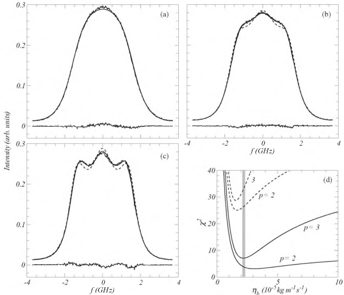
FIG. 4. N 2 spontaneous Rayleigh-Brillouin scattering for increasing pressures, p = 1, 2, and 3 bar for (a), (b), and (c), respectively. The dimensionless pressures are y = 0.60, 1.15, and 1.67 , respectively. Full lines correspond to model spectra computed using the Tenti S6 model, dashed lines correspond to model spectra using the Tenti S7 model. Lower full line indicates the difference between experiment and Tenti S6 model. (d) \chi^2 error as a function of bulk viscosity \eta_b ; full lines correspond to model spectra using the S6 model, dashed lines correspond to model spectra using the S7 model. The overall higher values of \chi^2 show that the spectra are not well described by the S7 model. The \chi^2 error at p = 3 using the S6 model has a minimum at \eta_b = 2.2 \times 10^{-5} \text{ kg m}^{-1} \text{ s}^{-1} , which is indicated by the grey line; the value of \eta_b at smaller pressures cannot be determined in this way.
