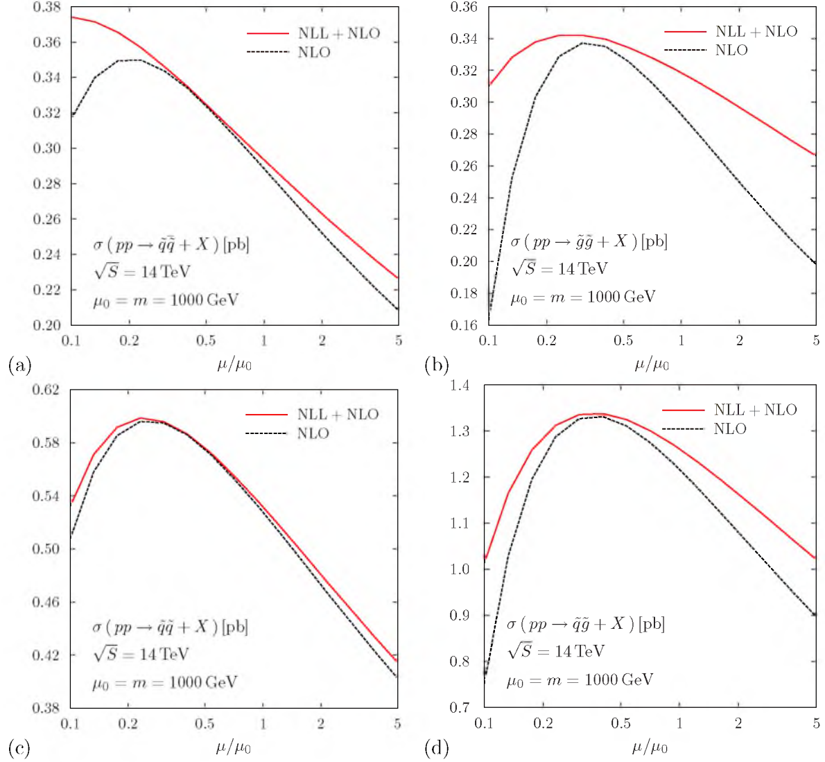
Figure 3: The scale dependence of the NLL+NLO and the NLO total cross sections for squark and gluino pair-production processes at the LHC. The squark and gluino masses have been set to m_{\bar{q}} = m_{\tilde{g}} = m = 1 TeV.
