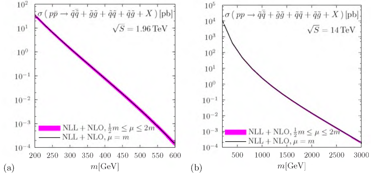
Figure 6: The NLL+NLO cross section for inclusive squark and gluino pair-production, pp/pp \rightarrow \bar{q}q + \bar{q}q + \bar{q}g + \bar{g}g + X , at the Tevatron (a) and the LHC (b) as a function of the average sparticle mass m . Shown are results for the mass ratio r = m_{\tilde{g}}/m_{\tilde{q}} = 1 . The error band corresponds to a variation of the common renormalization and factorization scale in the range m/2 \leq \mu \leq 2m .
