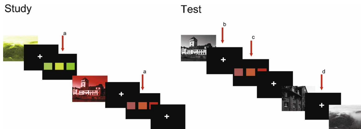
Figure 3. Simplified depiction of study and test trials. The letters a–d indicate whenever a button press had to be made. At a, subjects were required to indicate during study which color and shade of the color the pictures were dyed in. At b, subjects judged by button presses whether the photo was previously presented in red (old, previously red) or in green (old, previously green). If the subject judged the photograph to be old, previously red or old, previously green, subjects were required to indicate, at c, in which shade the photograph had been presented during the study phase. At d, subjects were required to press the button if they had not seen the photo before (new).
