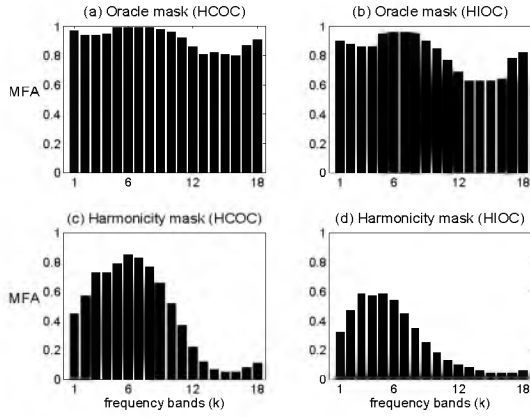
Figure 2. Example. The Mask Frame Average ( MFA ) of frames in the HCOC subset (a) and (c), and the HIOC subset (b) and (d). The sound class used to select the subset was the phone label /ah/. The MFA shows for every frequency band the fraction of frames that were considered reliable
