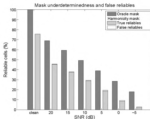
Figure 2: Percentage of reliable time-frequency cells for the oracle and harmonicity mask. The white areas indicate the portions that, according to the oracle mask, are falsely labeled reliable.
