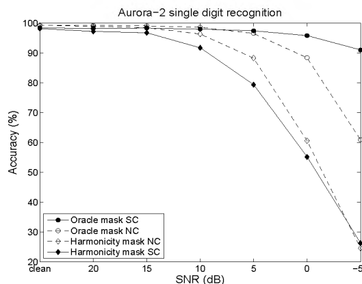
Figure 1: AURORA-2 single digit recognition accuracy. The figure shows results for both normal classification (NC) and sparse classification (SC) for the oracle mask and the harmonicity mask
