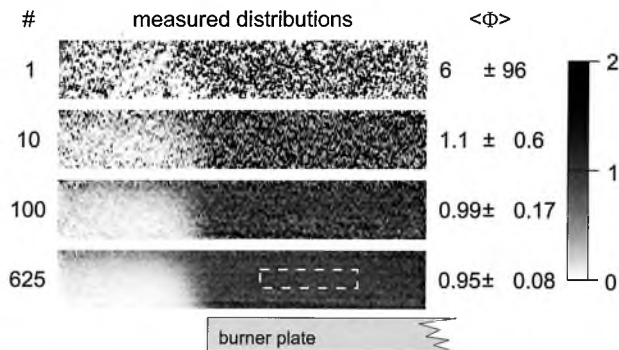
Fig. 10. Stoichiometry distributions determined from different numbers of laser shots. Spatial averages and standard deviations are determined in the dashed rectangular region (4050 pixels) of the stoichiometry for 625 laser pulses. See text for discussion.
