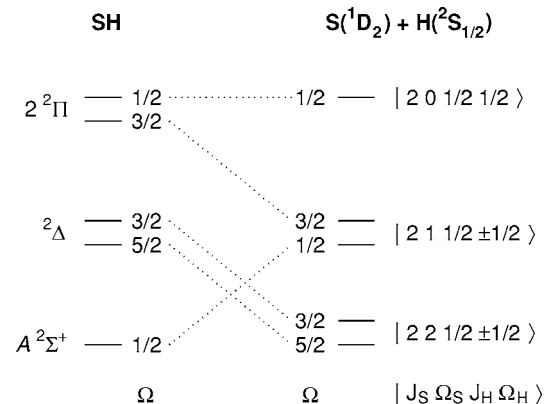
FIG. 2. Adiabatic correlation diagram for the \text{S}(^1D_2) + \text{H}(^2S_{1/2}) photodissociation channel of SH. The quantum number \Omega denotes the projection of the total electronic angular momentum with respect to the internuclear axis and correlates to \Omega_S + \Omega_H in the long range.
