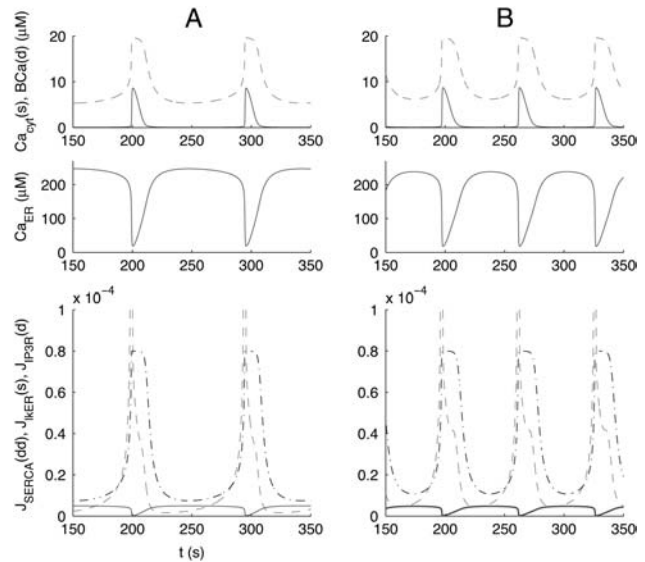
FIGURE 3 Simulation of the intracellular calcium oscillator for an IP 3 concentration of 0.5 \mu\text{M} (A) and 1 \mu\text{M} (B). When the IP 3 receptor opens, the calcium concentration in the ER decreases (A, middle panel), whereas the calcium concentration in the cytosol increases (A, solid line in upper panel). The buffer absorbs part of the calcium release in the cytosol (dashed line in upper panel). The lower panel of A shows the flow through the ER membrane. The flow of calcium ions through the IP 3 receptor during the opening of the IP 3 receptor (dashed line), the flow through the SERCA pump (dashed-dotted line), and the leak (solid line).
