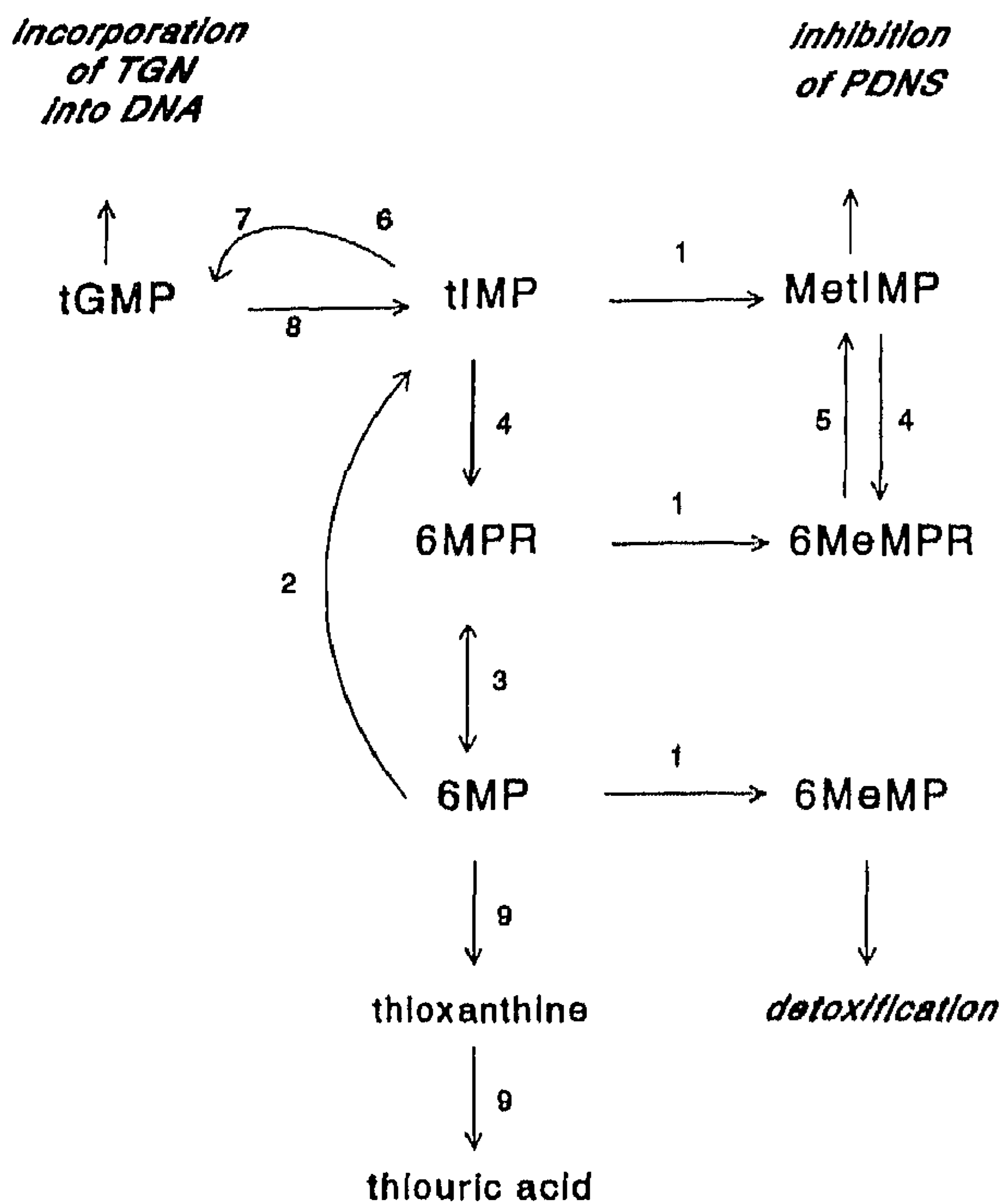
Fig. 1. Metabolism of 6-mercaptopurine. 6MP(R), 6-mercaptopurine-(riboside); 6MeMP(R), 6-methylmercaptopurine-(riboside); (Me)IMP, 6-(methylthioinosine monophosphate); tGMP, 6-thioguanosine monophosphate; PDNS, de novo synthesis of the purine. (1) thiopurine methyltransferase; (2) hypoxanthine guanine phosphoribosyltransferase; (3) purine nucleoside phosphorylase; (4) purine 5'-nucleotidase; (5) adenosine kinase; (6) inosine monophosphate dehydrogenase; (7) guanosine monophosphate synthetase; (8) guanosine monophosphate reductase; (9) xanthine oxidase.
