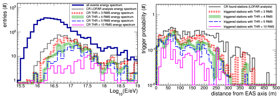
Figure 1. Left – Energy distribution of the LORA triggered dataset with “LBA outer” configuration: the whole set of showers (dark blue), the showers detected with the LOFAR off-line analysis (in black), and the showers detected with the self-trigger algorithm with threshold of 3 (red), 4 (green), 5 (blue), and 10 RMS (magenta). Right – Trigger probability for showers with energy above 2 \times 10^{17} eV and “LBA outer” configuration vs. the station distance from the shower axis for the LOFAR offline analysis (black) and the self-trigger algorithm with threshold 3 (red), 4 (green), 5 (blue), and 10 RMS (magenta).
