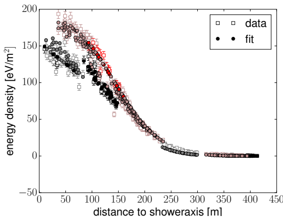
Figure 1. An example of a reconstructed air shower measured by LOFAR. The energy density is given as function of the distance to the shower axis. The colors indicate different azimuth angles. The red, pink, grey, and black points correspond to the northeast, southeast, southwest and northwest direction, respectively.
