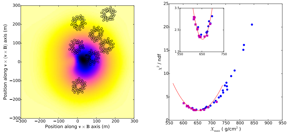
Figure 1. Left: event reconstruction. The small circles indicate LOFAR antenna positions (grouped in larger circles) projected into the shower plane. Their color reflects the measured power of the radio pulse. The background is a two-dimensional radio map from interpolated CoREAS simulations. The fit quality is high when the colors inside the circles blend into the background. Right: reconstruction of X_{\text{max}} . Every data point corresponds to a single simulated shower. Together they form the dedicated simulation set produced for this particular shower. The reduced \chi^2 of the fit is plotted against X_{\text{max}} and a parabola is fitted to find the reconstructed X_{\text{max}} . The inlay is a zoomed in version of the minimum of the curve demonstrating the sharpness of the minimum. Purple squares correspond to iron shower and blue circles to proton shower.
