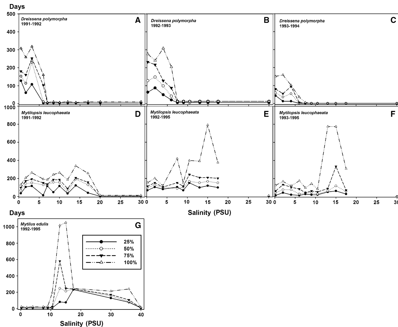
Fig. 2 Mortality (%) and survival (maximum number of days) of Dreissena polymorpha , Mytilopsis leucophaeata and Mytilus edulis at various salinities during various experimental periods
