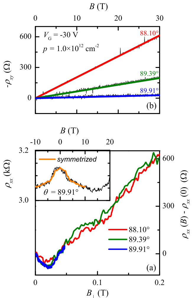
FIG. 2. Panel (a): Magnetoresistance at the CNP as a function of B_\perp at 1.4 K for three different angles \theta . The inset illustrates the symmetry of \rho_{xx} measured at \theta = 89.91^\circ with the black curve the original data between -10 T and 20 T and the orange line the symmetrized curve between -10 T and 10 T.
