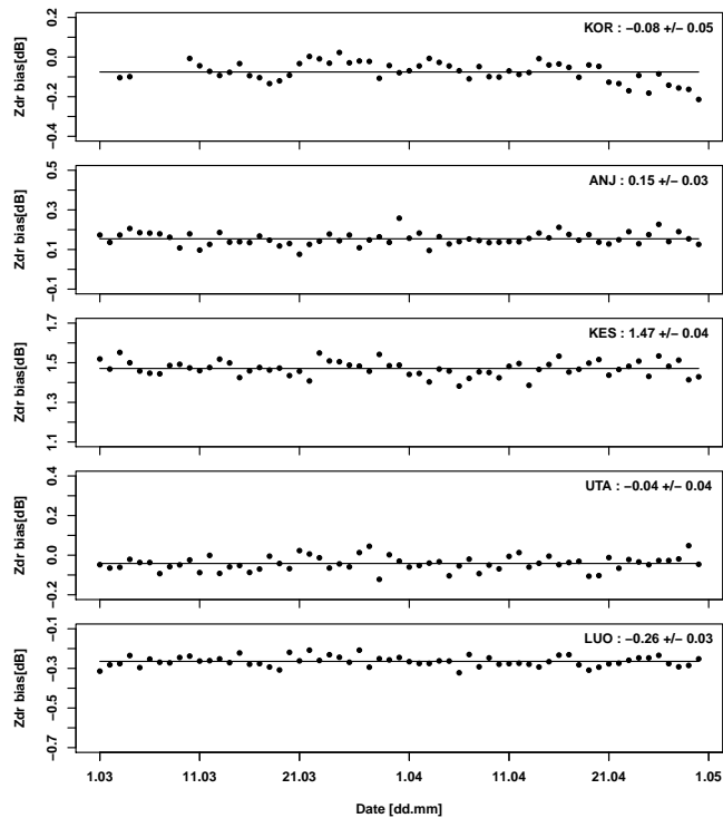
Figure 8. Z_{dr} results from solar signals for March and April 2015 for FMI radars indicated in the panels. The system Z_{dr} bias has not been subtracted from the data. The numbers in each panel give the mean and standard deviation for the data.
