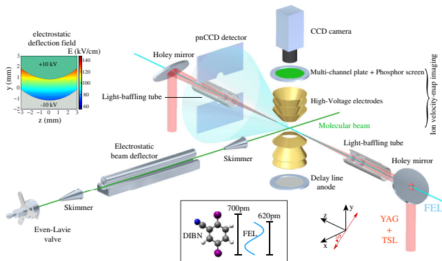
FIG. 1 (color online). Schematic view of the experimental setup: from the left, a supersonic beam with quantum-state selected molecules is delivered to the interaction point. In the center of a dual velocity map imaging spectrometer, the molecular beam is crossed by laser beams copropagating from right to left. The direct laser beams go through a gap in the pnCCD detectors that are used to record the diffraction pattern. The upper pnCCD panel is further away from the beam axis than the bottom panel in order to cover a wider range of scattering angles. In the inset, the molecular structure of 2,5-diiodobenzonitrile is depicted, together with a scale of its size, i.e., the iodine-iodine distance, and the wavelength of the x rays.
