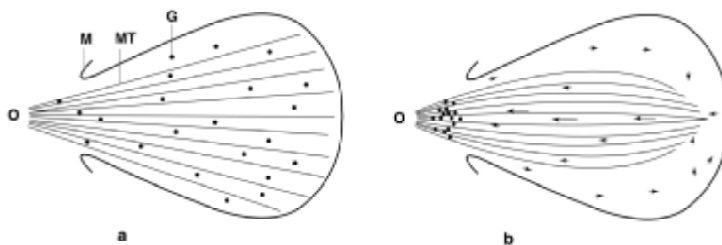
Fig. 2. Streaming-induced redistribution of pigment granules in the lobes of dermal chromatophores. a) Uniform distribution of granules (G) and microtubules at excess plus-end-directed motor activity. b) Granule aggregation and bundling of the distal microtubule domains caused by the plasma flow that is generated by the predominance of minus-end-directed motor activity. (O) Organization center of the aster-like arranged microtubules (plus-ends distal). Other symbols as in Fig. 1. For explanation see text.
