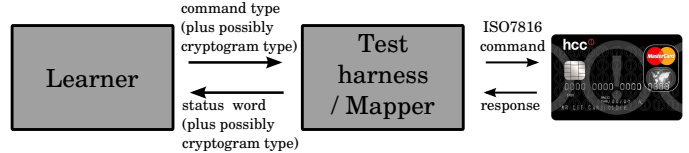
Fig. 2. Set-up
