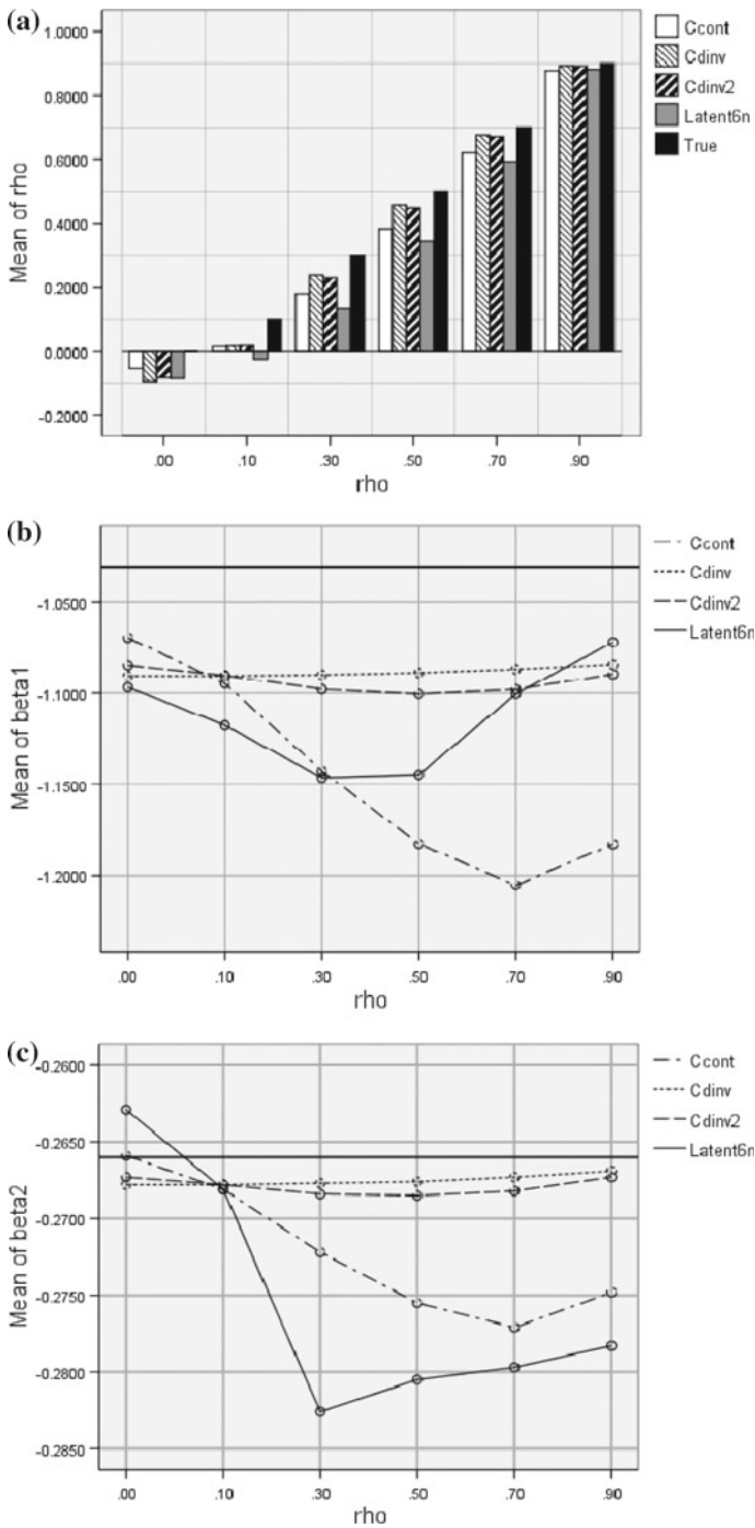
Fig. 3 Bias of the estimators of \rho (a), \beta_1 (b) and \beta_2 (c) for the classical models (Ccont, Cdiv, Cdiv2) and the latent model (Latent6n) for samples generated by inverse distance matrix
