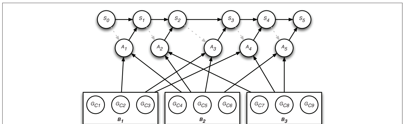
FIGURE A5 | An example of a Clique instance with k = 3 and |V| = 6 reduced to a RECEIVER instance. Here Boolean goal variables in the blocks encode vertices from the CLIQUE instance, actions encode "CLIQUE-rules" and states conjoin the rules. Degraded dependencies – i.e., those that have their conditional probabilities set such that they do not influence the Bayesian inference – are depicted by dotted arrows.
