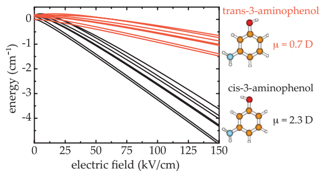
FIG. 2: (Color online) Molecular structures, dipole moments, and energies of the lowest rotational states of cis- and trans-3-aminophenol as a function of the electric field strength.
