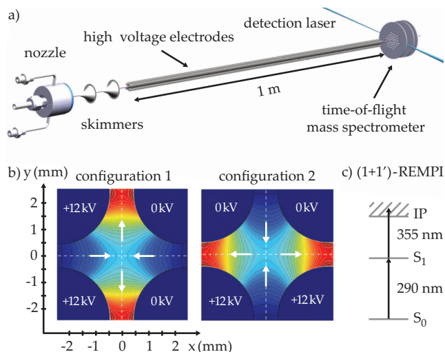
FIG. 1: (Color online) a) Scheme of the experimental setup. b) Cut through the high voltage electrodes and electric field configurations; red areas represent regions of strong electric field, blue areas regions of weak electric field. The electric field strength at the center is 45 kV/cm and contour lines are given every 4 kV/cm. White arrows indicate the direction of the force experienced by molecules in high-field seeking quantum states. c) Two color ionization detection scheme.
