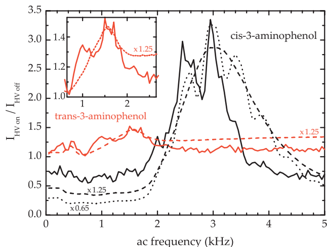
FIG. 3: (Color online) Experimental (solid lines) and simulated (dashed lines) transmission as a function of ac frequency for cis-3-aminophenol (black) and trans-3-aminophenol (red). The inset shows an enlarged view of the transmission curve of trans-3-aminophenol. The black dotted line represents simulations for cis-3-aminophenol that include the details of the detection process.
