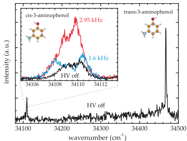
FIG. 4: (Color online) (1+1')-REMPI spectrum of 3-aminophenol. The spectrum is measured without high voltage applied to the selector, and shows the two origin transitions. In the inset, the rotational envelope of the cis-3-aminophenol origin transition is shown without high voltage (black) and with high voltage for ac frequencies of 2.95 kHz (red) and 1.6 kHz (blue).
