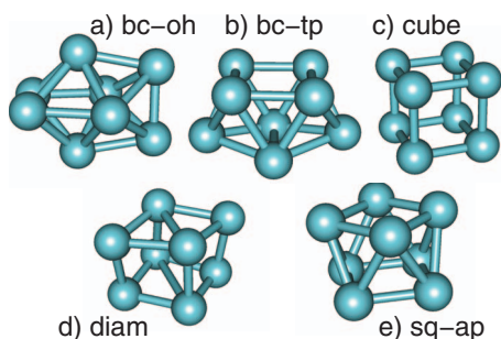
FIG. 2. Geometric structures of low-energy isomers of \text{Rh}_8^+ identified in DFT calculations: (a) bicapped octahedron (bc-oh), (b) bicapped trigonal prism (bc-tp), (c) cube, (d) diamond prism (diam), (e) square antiprism (sq-ap).
