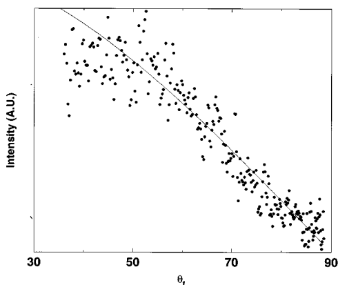
FIG. 9. In-plane angular distribution of scattered metastable CO molecules, as obtained from a 2D image as shown in Fig. 8. The circular points show the experimental data as obtained for a mixture of 20% CO in Ar, and an angle of incidence \theta_i = 33^\circ . The smooth curve shows a cosine distribution.
