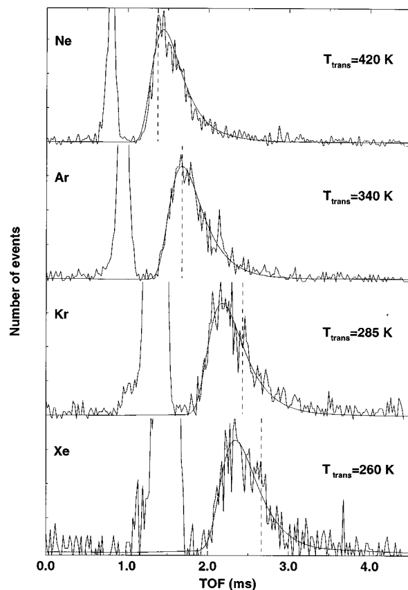
FIG. 6. Measured TOF profiles of scattered metastable CO molecules for mixtures of 20% CO in Ne, Ar, Kr and Xe. The best fit is superimposed upon the experimental traces. The dashed line, indicated for each of the TOF profiles, shows the averaged arrival time for a completely elastic scattering process, as obtained from the TOF distribution of the incoming beam.
