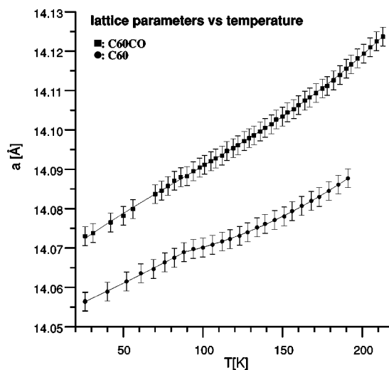
FIG. 1. The cubic lattice constant of (CO)_x C_{60} and C_{60} as a function of the temperature. The values were determined from the varying position of a single peak, and they were not corrected for the zero-point error. Error bars pertain to the standard deviations including the zero-point error. Relative values within one temperature run will be much more accurate, as the same zero-point error applies for all data points from a single run. The lines are a guide for the eye.
