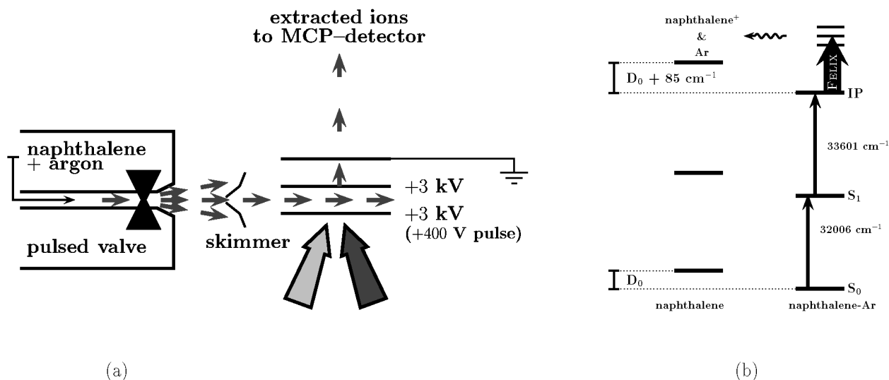
Fig. 1.—(a) Scheme of the experimental setup. (b) Excitation-ionization-dissociation scheme for monitoring the IR absorption spectrum of cationic naphthalene-Ar. Cluster cations are produced via (1+1′)-REMPI under field free conditions. IR-laser-induced dissociation of the ionic cluster is detected via the appearance of bare cationic naphthalene that is pulse-extracted several microseconds after ionization of the cluster.
