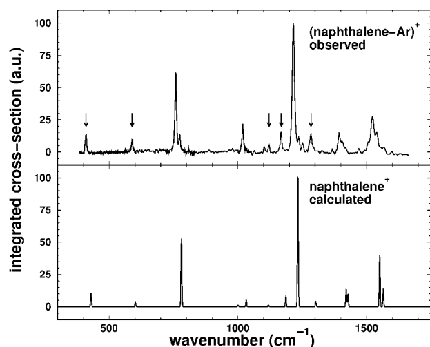
FIG. 2.— Top : Observed IR absorption spectrum of jet-cooled cationic naphthalene-Ar. Peaks not reported in matrix isolation experiments are marked with arrows. Bottom : Calculated IR absorption spectrum of cationic naphthalene.
