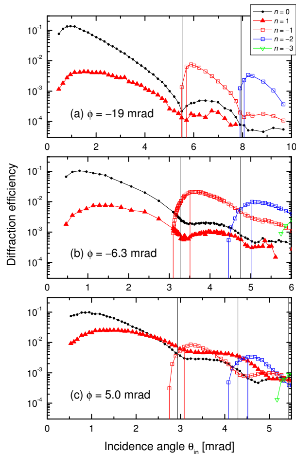
Figure 4. (Color online) Diffraction efficiencies measured at three azimuth angles: (a) \phi = -19 mrad; (b) \phi = -6.3 mrad; and (c) \phi = 5.0 mrad as a function of incidence angles \theta_{\text{in}} for T_0 = 8.7 K. The black vertical lines indicate the position of the Rayleigh angles of incidence where the -1 st and -2 nd order beams emerge. The boundaries of \Delta\theta_{R,m} are indicated by pairs of colored vertical lines.
