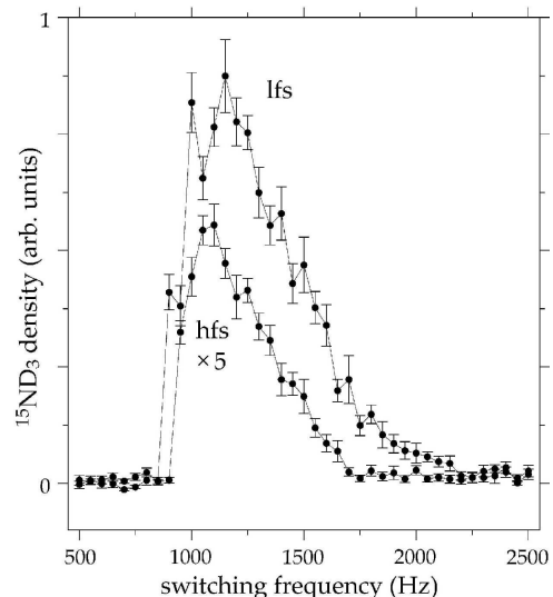
FIG. 3: Density of ^{15}\text{ND}_3 molecules in low-field seeking (lfs) and high-field seeking (hfs) levels of the |J, K\rangle = |1, 1\rangle state at the center of the trap as a function of the switching frequency, after the trap has been on for 72 ms. The signal of the high-field seekers is scaled up by a factor of 5.
