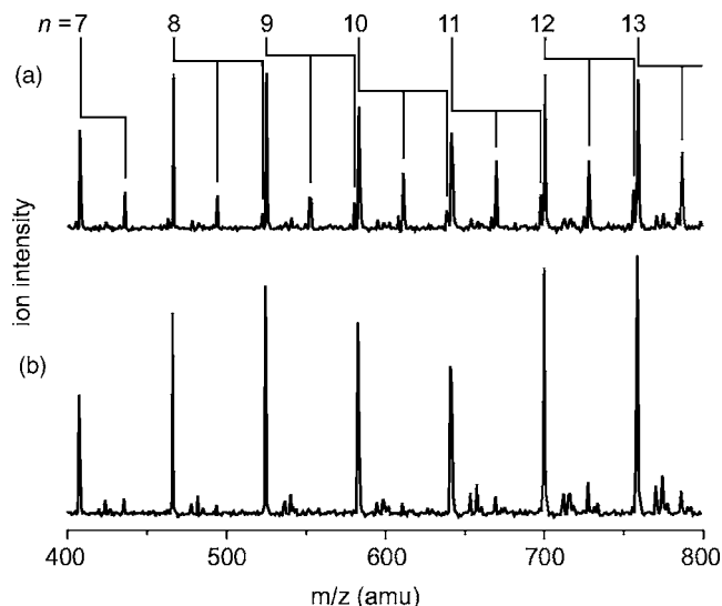
FIG. 1. Mass spectra demonstrating IR multiple photon dissociation of cationic cobalt cluster-CO complexes, \text{Co}_n(\text{CO})_m^+ . Spectrum (a) is obtained with the IR laser tuned to 1900 \text{cm}^{-1} , out of resonance with any IR band of the cationic complexes. Peaks due to \text{Co}_n(\text{CO})_1^+ and \text{Co}_n(\text{CO})_2^+ are identified by vertical bars. The spectrum is identical to that obtained with the IR laser turned off. Spectrum (b) is obtained with the IR laser tuned to 2000 \text{cm}^{-1} , in resonance with the CO stretching frequency, \nu(\text{CO}) , for many of the CO complexes in this mass range. Strong depletion of the \text{Co}_n(\text{CO})_m^+ mass peaks and growth of the bare \text{Co}_n^+ cluster peaks is apparent.
