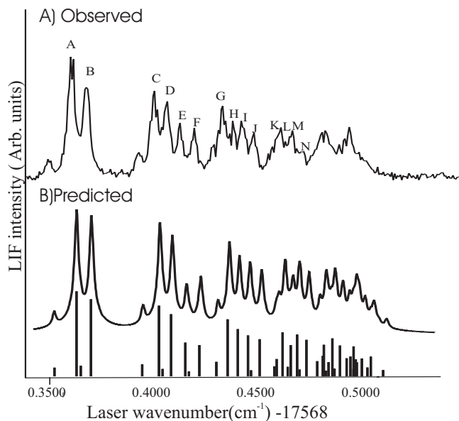
FIG. 1. The (a) observed and (b) calculated P_1(0) line ( \nu=17\,568.35\text{ cm}^{-1} ) of the A\ ^7\Pi_{2-} - X\ ^7\Sigma^+ (0,0) band of MnH, recorded under field-free conditions. There are a total of 43 transitions; the 14 most intense features are labeled and assigned in Fig. 2.
