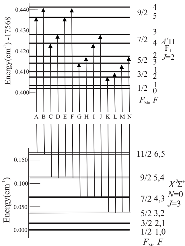
FIG. 2. The predicted field-free energy levels associated with the P_1(0) line ( \nu=17\,568.35\text{ cm}^{-1} ) of the A\ ^7\Pi_{2-} - X\ ^7\Sigma^+ (0,0) band of MnH. The 14 strongest transitions of Fig. 1 are indicated. The energy scale for the A\ ^7\Pi state has been expanded by a factor of 4 relative to that of the X\ ^7\Sigma^+ state.
