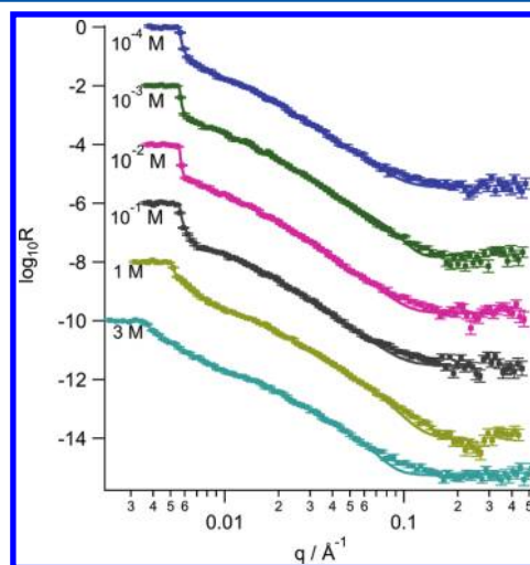
Figure 4. Neutron reflectivity from poly(METAC) brush in increasing concentrations of KNO_3 in D_2O . Symbols show measured data; solid lines show fits to two-region model (for parameter values, see the Supporting Information). Successive profiles are shown displaced vertically for clarity. The shifted critical edges at 1 and 3 M are due to the changed refractive index of the aqueous subphase.
