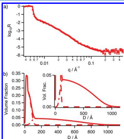
Figure 3. Two-region structure of poly(METAC) brush in pure water ( D_2O ). (a) Neutron reflectivity, R , as a function of momentum transfer, q . Symbols show measured data; solid line shows fit to two-region model (for parameter values see Supporting Information). (b) Polymer volume fraction of profile corresponding to solid-line fit in a. Solid line (—) shows total volume fraction; dashed line (--) shows polymer associated with surface region, and dashed-dotted line (-·-) shows the brush region.
