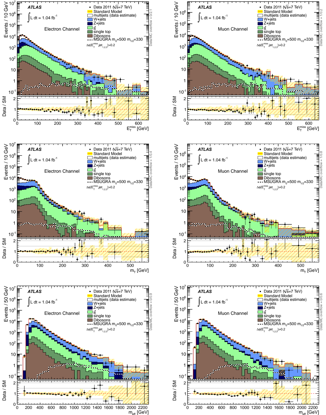
FIG. 1: Distributions after requiring one electron with p_T > 25 \text{ GeV} or one muon with p_T > 20 \text{ GeV} , and at least three jets with p_T > 60, 25, 25 \text{ GeV} and \Delta\phi(\text{jet}_i, \vec{E}_T^{\text{miss}}) > 0.2 . The top row shows the missing transverse momentum, E_T^{\text{miss}} , the middle row shows the transverse mass, m_T , and the bottom row displays the effective mass, m_{\text{eff}} . The electron channel is shown in the left column, the muon channel is shown in the right column. The “Data/SM” plots show the ratio between data and the summed standard model expectation. In these plots, the standard model expectation is derived from Monte Carlo simulations only, normalized to the theoretical cross sections. The uncertainty band on the standard model expectation combines the MC statistical uncertainty and systematic uncertainties on the jet energy scale and resolution, the lepton resolution and identification efficiencies, pile-up and luminosity. For illustration, the expected signal distributions of the MSUGRA/CMSSM model point m_0 = 500 \text{ GeV} , m_{1/2} = 330 \text{ GeV} are also shown.
