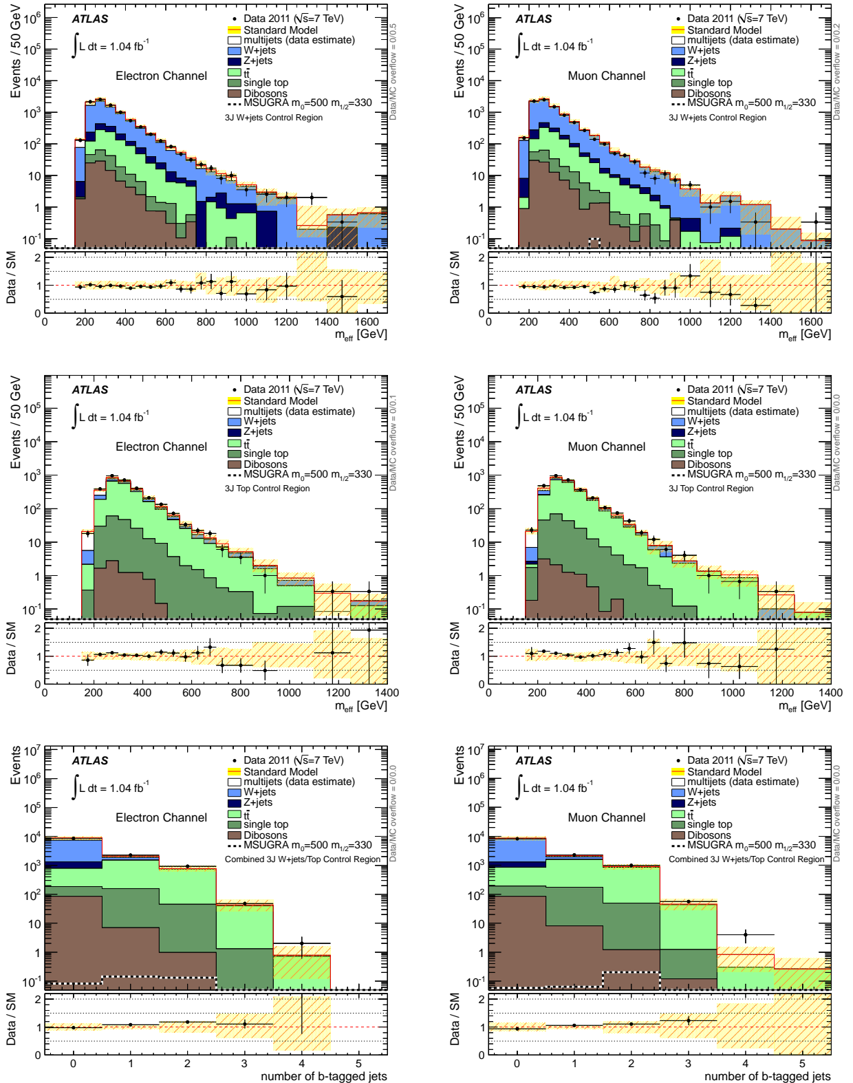
FIG. 3: Distributions for events in the lepton plus three jets control regions for the electron channel (left column) and muon channel (right column). Top row: effective mass in the W+jets control region. Middle row: effective mass in the top control region. Bottom row: number of b -tagged jets in the combined W+jets and top control regions. The “Data/SM” plots show the ratio between data and the summed standard model expectation. The uncertainty band on the standard model expectation combines the MC statistical uncertainty and systematic uncertainties on the jet energy scale and resolution, b -tagging, the lepton resolution and identification efficiencies, pile-up and luminosity.
