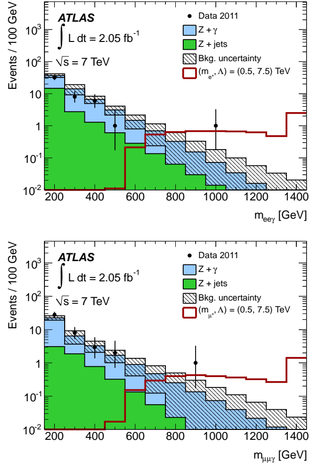
FIG. 6: Distributions of the invariant mass for the \ell\ell\gamma system for the e^* (top) and \mu^* (bottom) searches after requiring m_{\ell\ell} > 110 GeV. The Z + jets and Z + \gamma backgrounds were fitted, and the total uncertainties from the fit as well as the uncertainty in the Z + jets normalization measured in the control region are displayed as the shaded area. Note that the last bin contains the sum of all events with m_{\ell\ell\gamma} > 1450 GeV.
