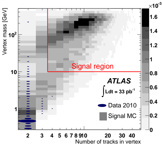
Figure 7: Vertex mass ( m_{\text{DV}} ) vs. vertex track multiplicity ( N_{\text{DV}}^{\text{trk}} ) for displaced vertices in events that pass the selection requirements except the m_{\text{DV}} and N_{\text{DV}}^{\text{trk}} requirements, which are not applied. Shaded bins show the distribution for the signal MC MH sample (see Table 1), and data are shown as filled ellipses, with the area of the ellipse proportional to the number of vertices in the corresponding bin. The figure contains 487 data vertices, of which 251 are in the bin corresponding to K_S^0 decays.
