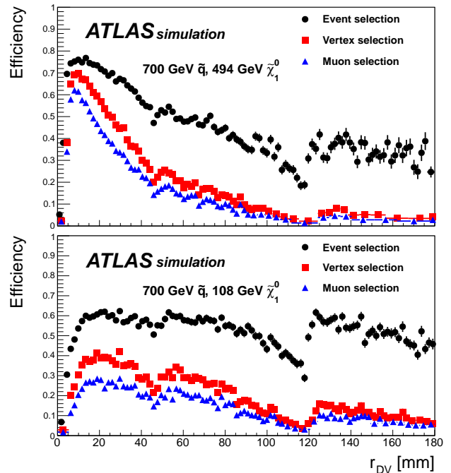
Figure 3: The efficiency as a function of r_{\text{DV}} for vertices in the signal MC samples MH (top) and ML (bottom) of Table 1. In each plot, the top histogram (circles) is the efficiency for the event selection criteria, the middle histogram (squares) shows the efficiency when also requiring one vertex to satisfy the vertex-selection criteria, and the bottom histogram (triangles) includes the muon-selection criteria. The material veto is not applied when making these plots.
