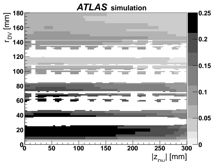
Figure 4: The efficiency as a function of r_{\text{DV}} and z_{\text{DV}} for vertices in the signal MC sample ML of Table 1. High-density material regions that are vetoed are shown in white. The four major vetoed regions surround the beampipe wall, at radii of about 25 – 37 mm, and the three barrel pixel layers.
