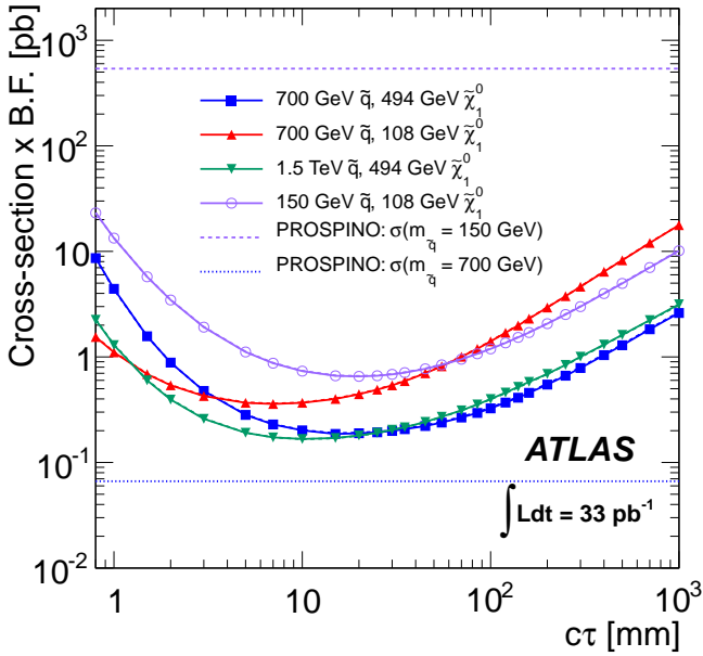
Figure 8: Upper limits at 95% CL on the production cross-section times branching fraction vs. the neutralino lifetime times the speed of light for different combinations of squark and neutralino masses, based on the observation of zero events satisfying all criteria in a 33 \text{ pb}^{-1} data sample. The horizontal lines show the cross-sections calculated from PROSPINO for squark masses of 700 GeV and 150 GeV.
