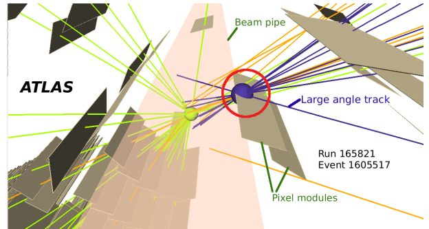
Figure 2: An event from a jet-trigger data sample, where a high-mass vertex (circled) is the result of an apparently random, large-angle intersection between a track (labeled as “Large angle track”) and a low- m_{DV} hadronic-interaction vertex produced in a pixel module. Tracks originating from this vertex are shown in blue, those from the primary vertex are green, and other tracks are orange. The beampipe and pixel modules with track hits are shown.
