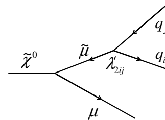
Figure 1: Example of a diagram of a new massive particle \tilde{\chi}^0 (such as the lightest neutralino) decaying into a muon and two jets via a virtual smuon, with lepton-number and R -parity violating coupling \lambda'_{2ij} .
