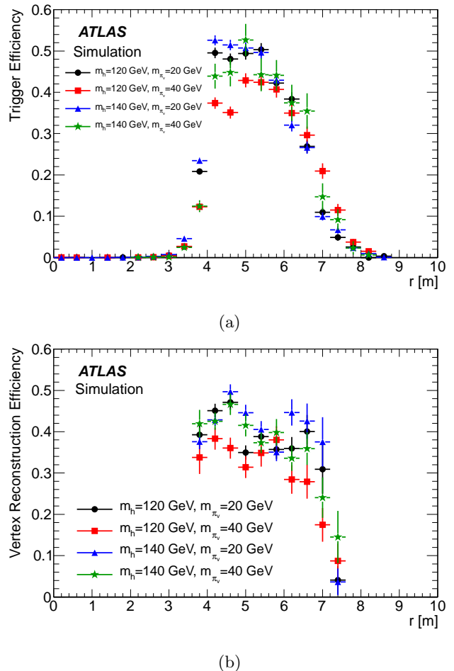
FIG. 1: a: Efficiency of the trigger, as a function of the radial decay position ( r ) of the \pi_\nu . b: The vertex reconstruction efficiency for \pi_\nu decays in the barrel for events that pass the muon RoI cluster trigger as a function of the radial decay distance. The error bars represent the statistical uncertainty on the efficiencies.
