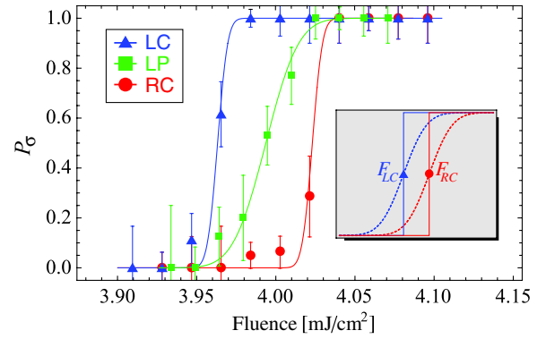
FIG. 1 (color online). Switching probability P_\sigma as a function of the fluence at \lambda = 700 nm for three different polarizations. The measurements with RC and LC pulses were performed at a different time than the ones with LP pulses, and therefore the laser stability \epsilon was different. Inset: Illustration of the switching probabilities in case of zero (solid) and nonzero (dashed) laser fluctuations using Eq. (1). F_{LC} and F_{RC} denote the switching threshold of GdFeCo for LC and RC excitation pulses, respectively.
