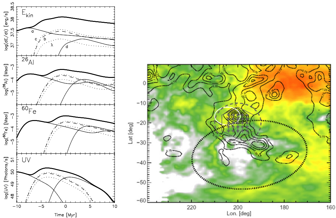
Figure 1. Left: Our simulated output of kinetic energy, ^{26}\text{Al} , ^{60}\text{Fe} and ionizing radiation from the massive stars in the Orion region. The thin lines indicates the outputs from the individual regions of the Orion OB1 association. It can be seen that the radioactive elements are good tracers of the kinetic energy output, making them useful for the study of feedback from massive stars. The results were shown to be consistent with observed properties of the region: ISM excavation by the kinetic energy, free-free emission from the ionized ISM and gamma-rays from the radioactive decay of ^{26}\text{Al} . Right: The COMPTEL-observed 1.8 MeV emission (contours), superimposed on a velocity integrated HI map of Orion-Eridanus bubble (color image). Orion OB1 is indicated (white ellipse), as well as the outer shell of the HI superbubble (large, black-dotted ellipse).
