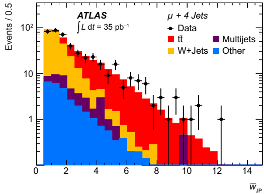
Figure 3: Input variables to the likelihood discriminants in the exclusive four-jet bin for the muon channel: lepton \eta (top), \exp(-8 \times \mathcal{A}) (second from top), \exp(-4 \times H_{T,3p}) (third from top) and \bar{w}_{JP} (bottom). All simulated processes are normalized to theoretical SM predictions, except the multijet background which uses the normalisation presented in Sec. 6. These distributions are used in the tagged analysis.
