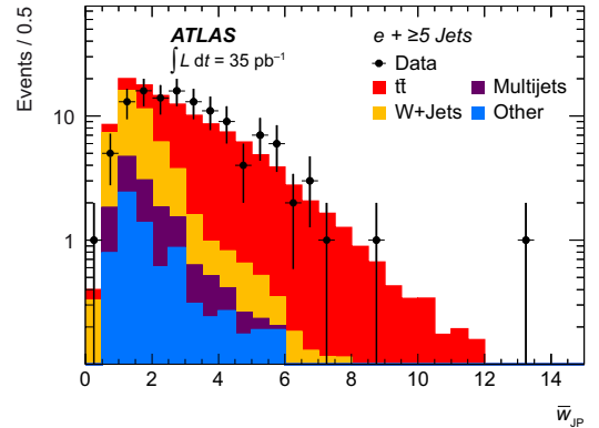
Figure 4: Input variables to the likelihood discriminants in the inclusive five-jet bin for the electron channel: lepton \eta (top), \exp(-8 \times \mathcal{A}) (second from top), \exp(-4 \times H_{T,3p}) (third from top) and \bar{w}_{JP} (bottom). All simulated processes are normalized to theoretical SM predictions, except the multijet background which uses the normalisation presented in Sec. 6. These distributions are used in the tagged analysis.
