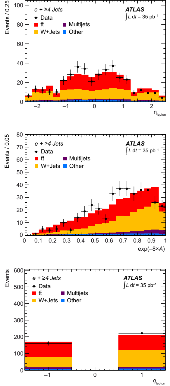
Figure 2: Input variables to the likelihood discriminants in the inclusive four-jet bin for the electron channel: lepton \eta (top), \exp(-8 \times \mathcal{A}) (middle) and lepton charge (bottom). All simulated processes are normalized to theoretical SM predictions, except the multijet background which uses the normalisation presented in Sec. 6. These distributions are used in the untagged analysis.
