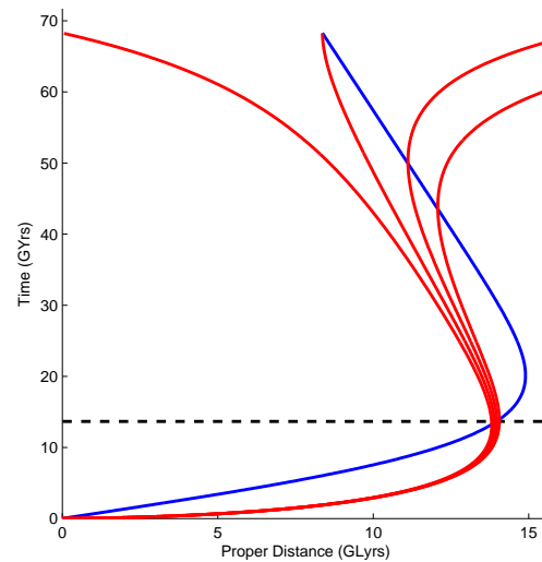
Figure 4. As Figure 3, but considering photon paths that do not necessarily reach the origin.
