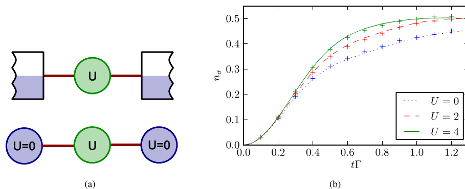
Figure 6 (online color at: www.ann-phys.org ) (a) Model under consideration: a quantum dot (interacting impurity) is coupled to two infinite reservoirs at half filling. The time-dependence is given by a sudden switch in the tunneling to the reservoirs to a non-zero value at t = 0 . The reference system is a single impurity with the
