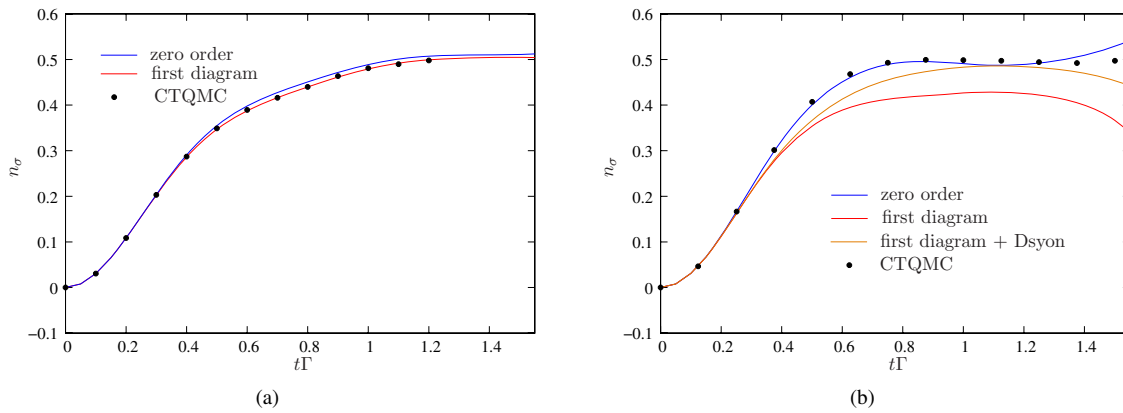
Figure 7 (online color at: www.ann-phys.org ) Same system as on Fig. 6 with the inclusion of the first diagram. (a) U = 2 , (b) U = 8 . For the case (b) results with and without taking Dyson equation for the dual Green function into account are shown.
