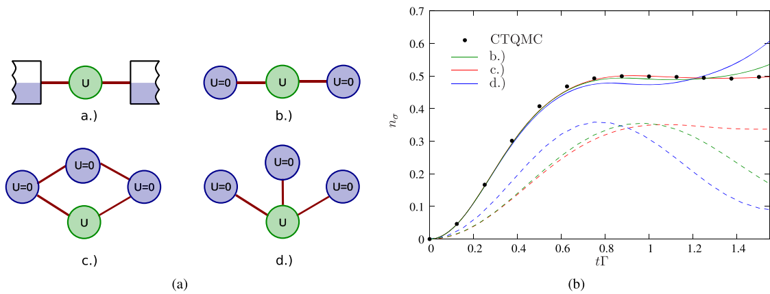
Figure 8 (online color at: www.ann-phys.org ) Investigation of the influence of the reference system on the result of the dual perturbation expansion. Left: Models under consideration: (a) quantum dot (interacting impurity) coupled to two infinite reservoirs at half filling. The dot is empty for t < 0 . (b–d) different reference systems considered as a starting point for the dual expansion. Right: Comparison of the occupation of the dot in lowest order dual approximation (see Eq. (30)) (lines) to CT-QMC data (dots) for U = 8 . The temperature is \beta\Gamma = 10 . Dashed lines show the time evolution of the corresponding Hamiltonian reference systems.
