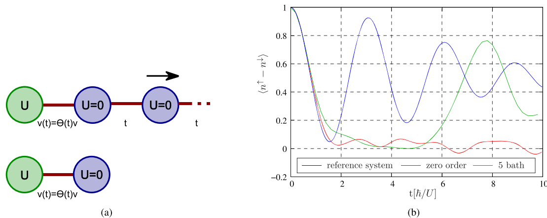
Figure 5 (online color at: www.ann-phys.org ) (a) An infinitely long chain with one interacting impurity at the left end is approximated by an effective two sites model with the same parameters. The initial state is prepared by a single spin on the impurity. The time-dependence is given by a sudden switch in the hopping to the rest
