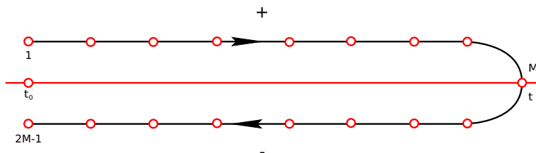
Figure 1 (online color at: www.ann-phys.org ) Illustration of the Keldysh contour: the contour starts and ends at t_0 . Times are ordered in such a way, that points on the lower branch (-) are always later than points on the upper branch (+).
