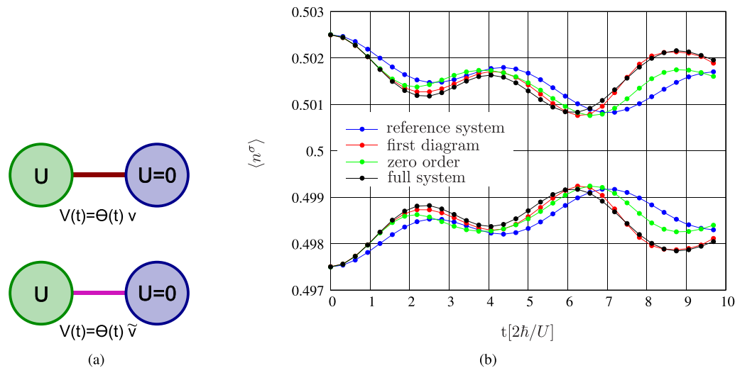
Figure 3 (online color at: www.ann-phys.org ) Simple test of the superperturbation method on the Keldysh contour. (a) the model under consideration consists of one interacting site coupled to one bath site (upper left picture), with the energy level of the interacting impurity fixed to -U/2 and the level of the bath to zero. The time dependence consists of a sudden switch in the hopping amplitude from an infinitesimally small value to a non-zero one. The reference system is prepared in the same way, but the hopping is switched to a lower value (lower left picture). (b) Plot of the occupation probability n^\sigma(t) for spin up (upper curve) and down
