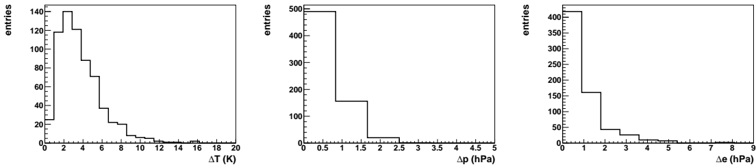
Figure 2: Differences between maximum and minimum values for temperature T , pressure p , and water vapor pressure e as found in weather station data during a weather balloon launch. For temperature data (left), typical conditions are defined as variances between 4 K and 9 K, with 4 K being \Delta Q_{\text{low}} for the quantity temperature. Periods with \Delta T < 4 K indicate very stable conditions while periods with \Delta T > 9 K are unstable. For pressure data (middle), typical conditions are defined between 1 and 3 hPa. For water vapor pressure data (right), the typical conditions are between 0.8 and 4.0 hPa. The very stable and unstable conditions of the last two quantities are defined accordingly.
