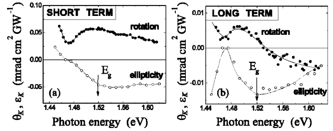
FIG. 5. Spectral dependence of the Kerr rotation \theta_K and ellipticity \varepsilon_K in CdTe (a) in the short term and (b) in the long term for pump-probe delays corresponding to the solid arrows in Fig. 4. Lines are guides to the eye.
