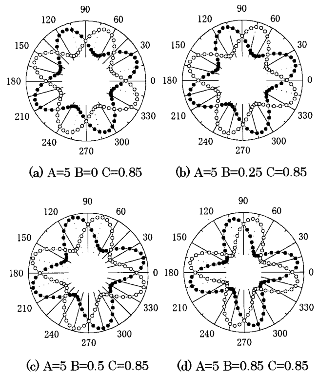
FIG. 4. Analyzer angle dependence of SH signal in Fe(3.75 ML)/Au(3.75 ML) superlattice for two opposite directions of the magnetic field.
