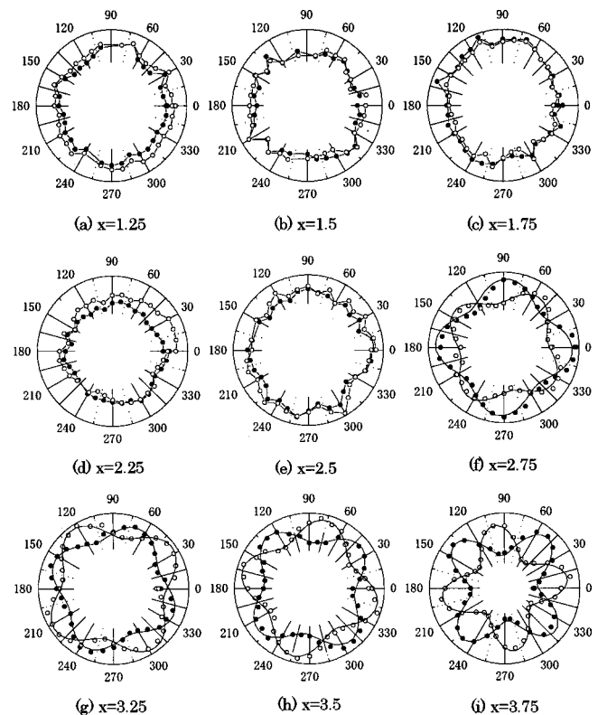
FIG. 2. Polar plots of azimuthal patterns of MSHG signal in superlattices with (a) x=1.25 , (b) x=1.5 , (c) x=1.75 , (d) x=2.25 , (e) x=2.5 , (f) x=2.75 , (g) x=3.25 , (h) x=3.5 , and (i) x=3.75 .
