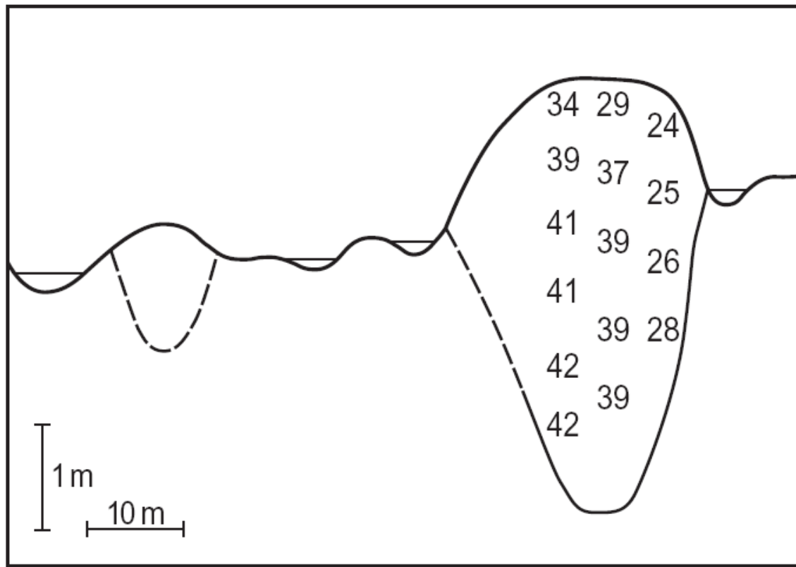
Figure 10. Temperature profiles ( ^{\circ}\text{C} ) in the large cupola in Mfayeni. Warm water was rising very high in the peat dome and cooled down only in the top 0.2 m. We were unable to investigate the dry cupola(s) shown on the left-hand side with the temperature probe, due to the high penetration resistance of the soil.
