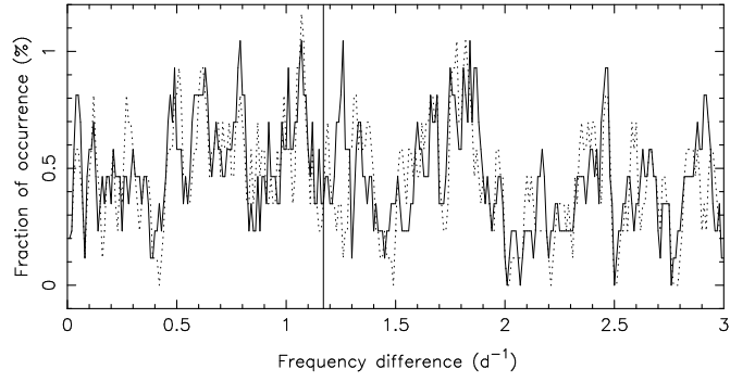
Fig. 6. Fraction of the occurrence of values for the frequency differences between zonal p modes of degree \ell = 0, \dots, 4 in the frequency regime [11, 26] \text{ d}^{-1} compared with the spacing of 1.17 \text{ d}^{-1} reported by Belkacem et al. (2009). The full line is for the model of 11.4 M_{\odot} , while the dotted line is for the model with 11.7 M_{\odot} indicated in italics in Table 2.
