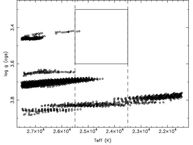
Fig. 2. Kiel diagram showing all the models with a radial mode at the frequency 5.48694 \text{d}^{-1} excited and matching the additional eight higher mode frequencies listed in Table 1. The 1\sigma error box for the spectroscopically derived T_{\text{eff}} and \log g is shown as well. The dashed vertical lines indicate the restriction we imposed on the models.
