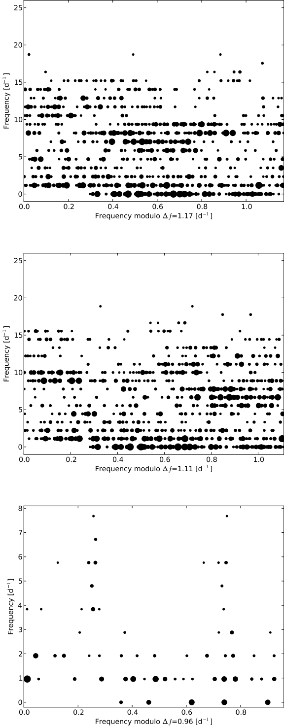
Fig. 5. Échelle diagrams of the CoRoT frequencies for HD 180642 for the large spacing determined by Belkacem et al. (2009, upper panel) and in Paper I (middle panel). For comparison, we also show the échelle diagram of the O8.5V star HD 46149 reproduced from Degroote et al. (2010b), where clear ridges produced by stochastically excited modes are found. The size of the symbols scales with the power of the frequency.
