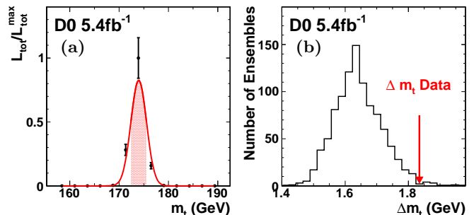
FIG. 2: Combined for all channels: (a) Calibrated and normalized likelihood for the data as a function of m_t with the best estimate as well as 68% confidence level region marked by the shaded area and in (b) the expected distribution of uncertainties with the measured uncertainty indicated by the arrow. As the top quark mass is measured to be m_t = 174.0 \text{ GeV} , the expected distribution in (b) is shown for the closest input mass m_t = 175 \text{ GeV} used in the pseudoexperiment.
