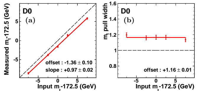
FIG. 1: (a) Mean values of m_t and (b) pull width from sets of 1000 pseudoexperiments as a function of input m_t for the combined dilepton channels. The dashed lines represent the ideal response in (a), where the extracted mass is identical to the input mass, and in (b), where the statistical uncertainty requires no correction.
